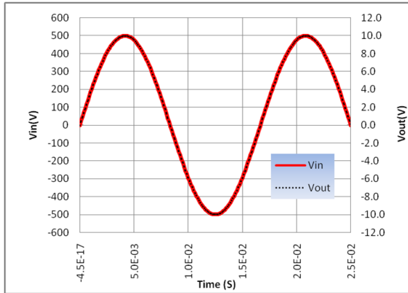
Figure 7: 60Hz Response
