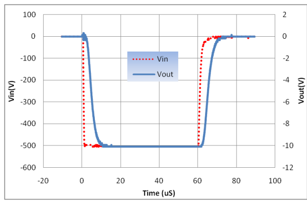
Figure 14: -500V Input Step Response
