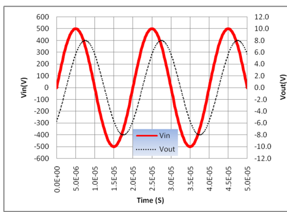
Figure 12: 50KHz Response
