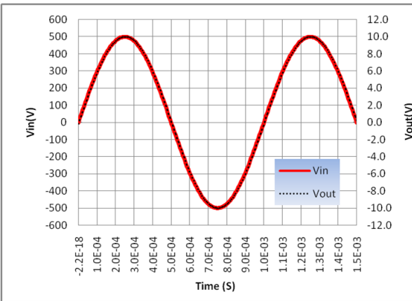
Figure 9: 1KHz Response
