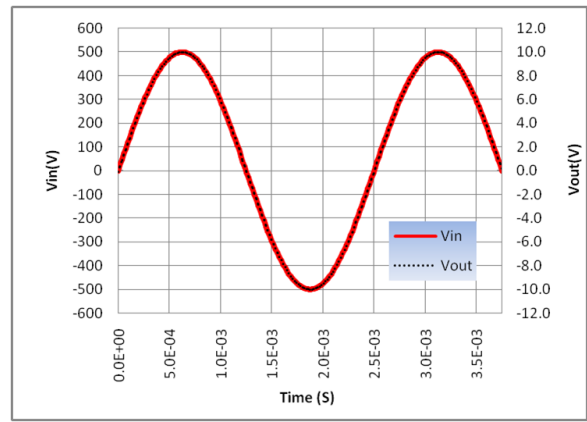
Figure 8: 400Hz Response
