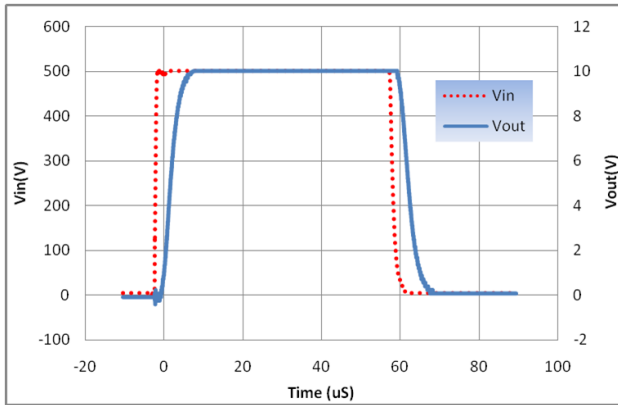
Figure 13: 500V Input Step Response
