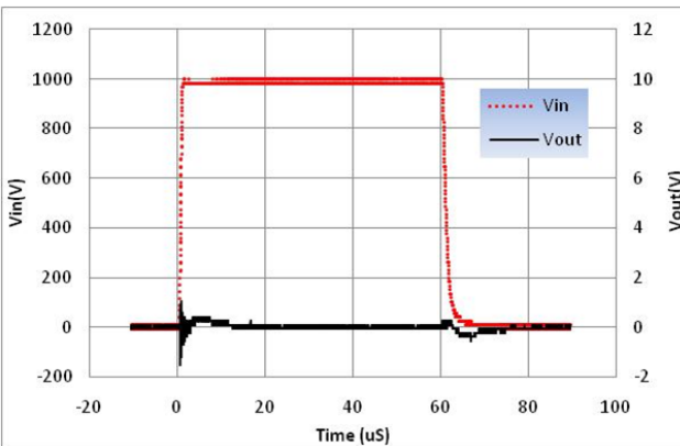
Figure 15: 1000V Common Mode Rejection Response
