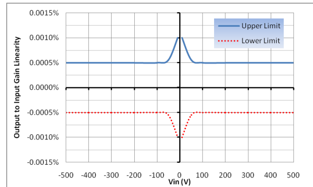
Figure 4: Gain Nonlinearity
