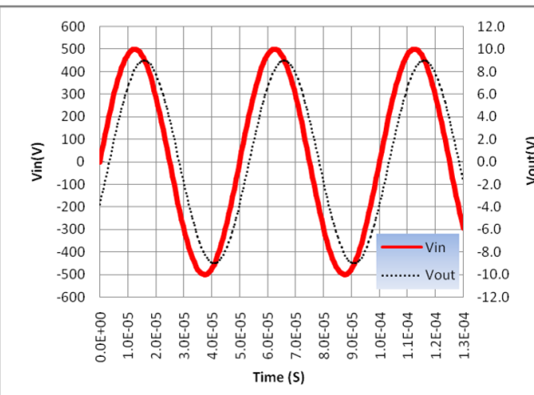
Figure 11: 20KHz Response
