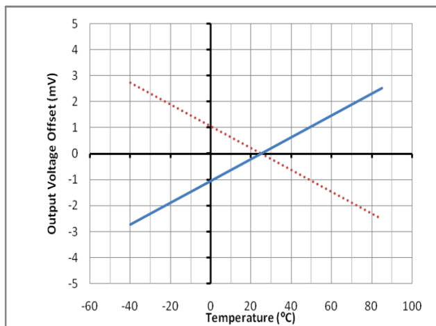
Figure 5: Output Voltage Drift vs. Temperature
