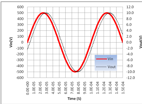
Figure 10: 10KHz Response
